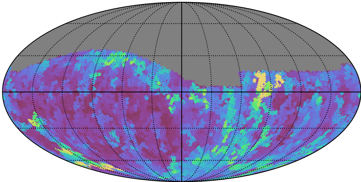
ddf_loaded_fl2_v3.4_10yrs Yr 1 g band: Max seeingEff
