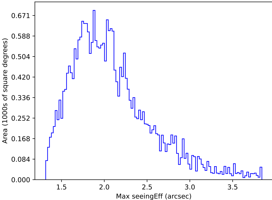
ddf_loaded_fl2_v3.4_10yrs Yr 1 all bands: Max seeingEff
