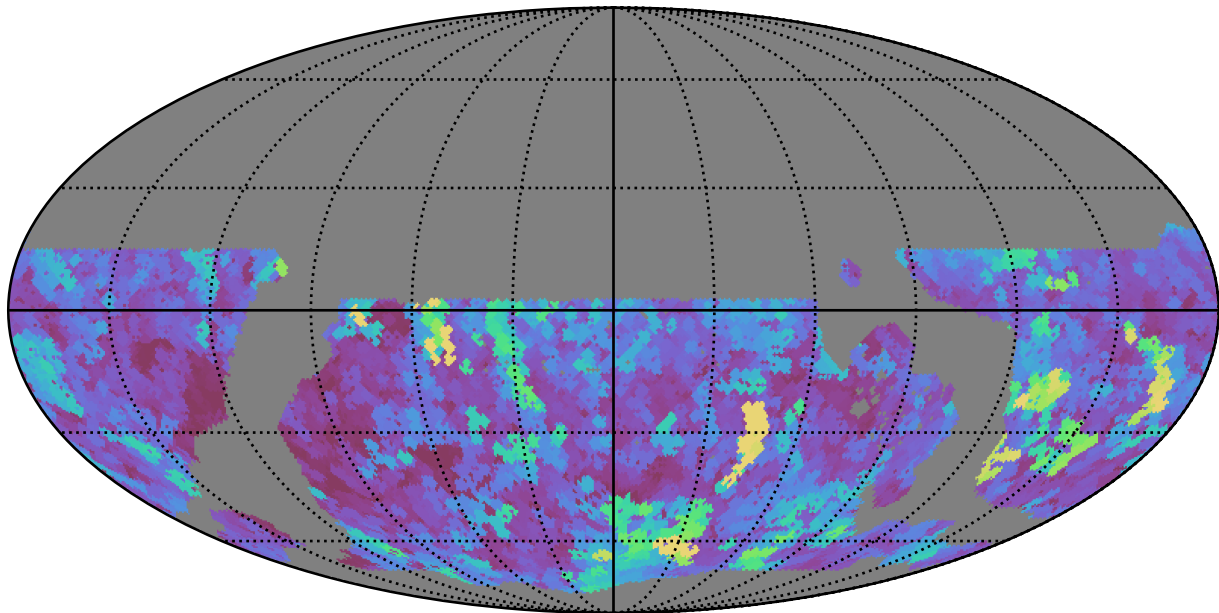
ddf_loaded_fl2_v3.4_10yrs WFD z band: Max seeingEff
