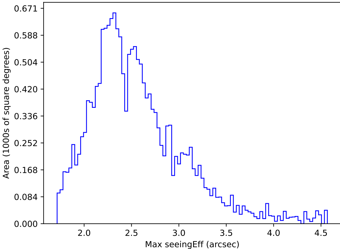
ddf_loaded_fl2_v3.4_10yrs WFD z band: Max seeingEff
