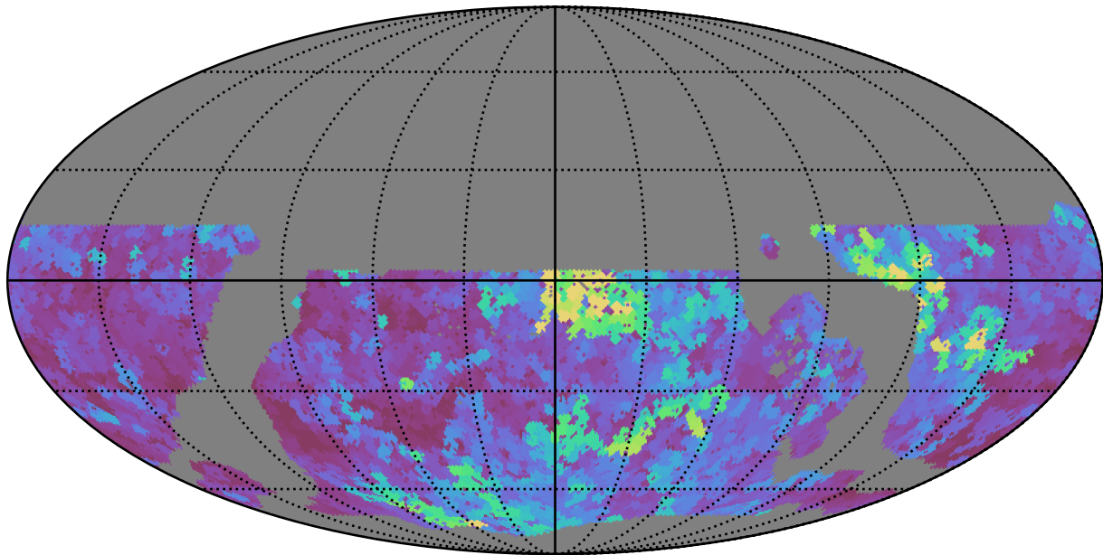
ddf_loaded_fl2_v3.4_10yrs WFD y band: Max seeingEff
