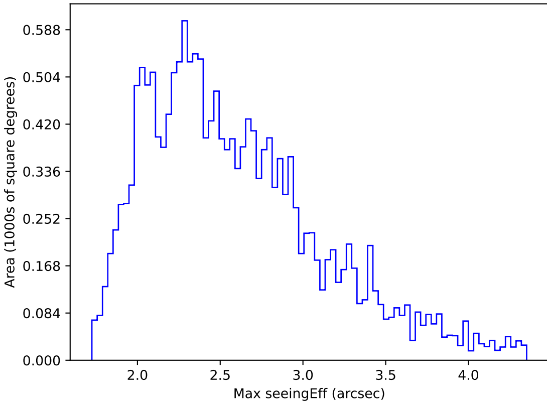
ddf_loaded_fl2_v3.4_10yrs WFD u band: Max seeingEff
