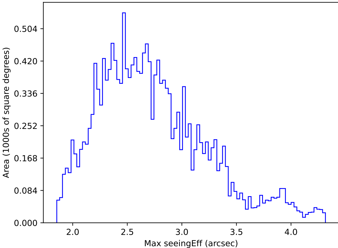
ddf_loaded_fl2_v3.4_10yrs WFD r band: Max seeingEff
