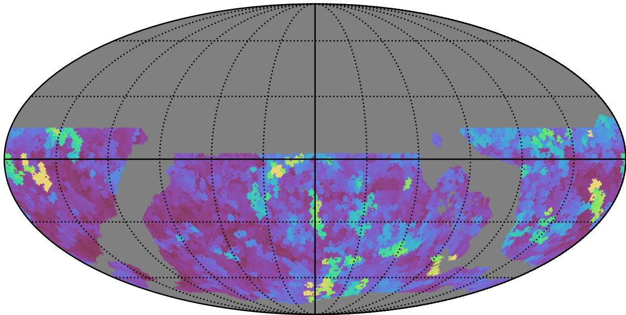
ddf_loaded_fl2_v3.4_10yrs WFD i band: Max seeingEff
