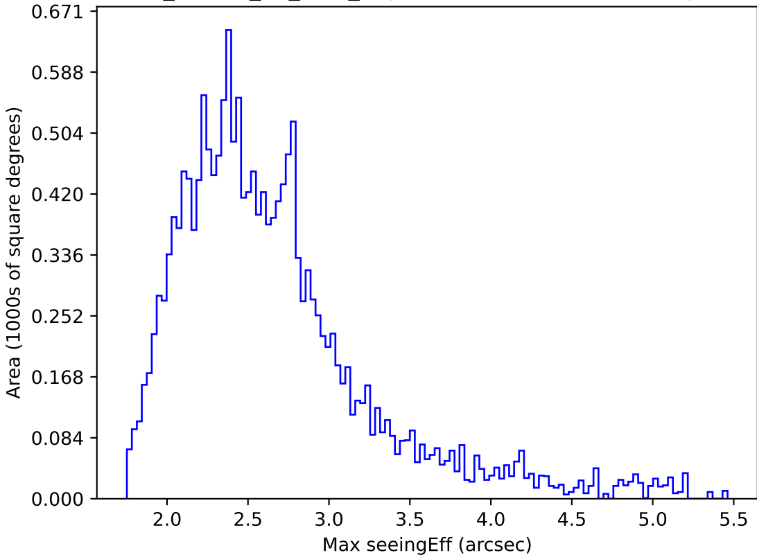
ddf_loaded_fl2_v3.4_10yrs WFD i band: Max seeingEff
