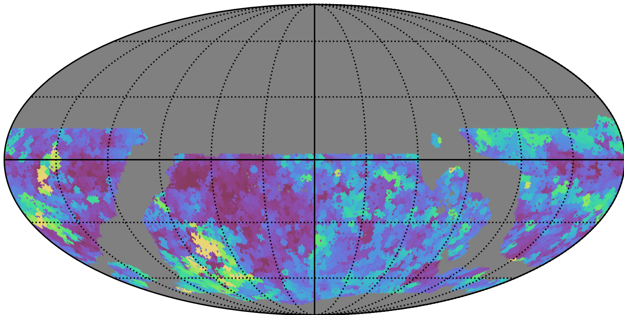
ddf_loaded_fl2_v3.4_10yrs WFD g band: Max seeingEff
