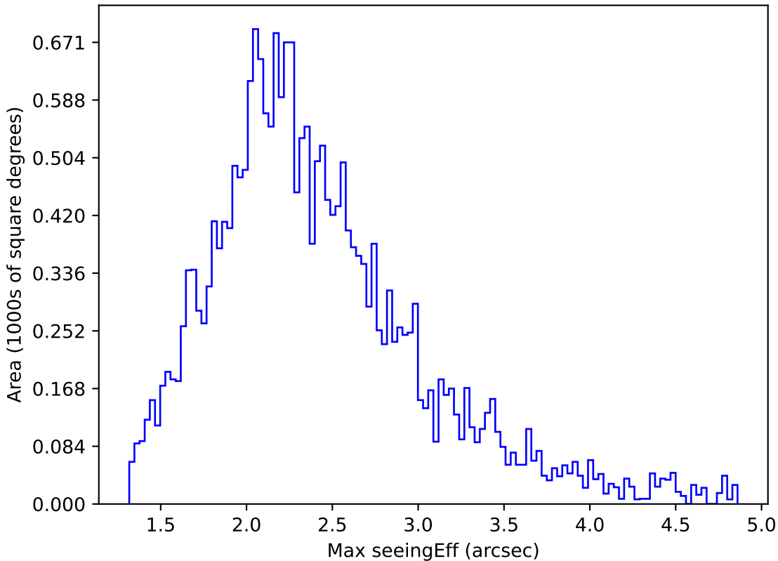
ddf_loaded_fl2_v3.4_10yrs All sky y band: Max seeingEff
