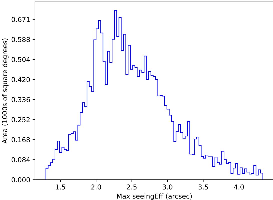
ddf_loaded_fl2_v3.4_10yrs All sky u band: Max seeingEff
