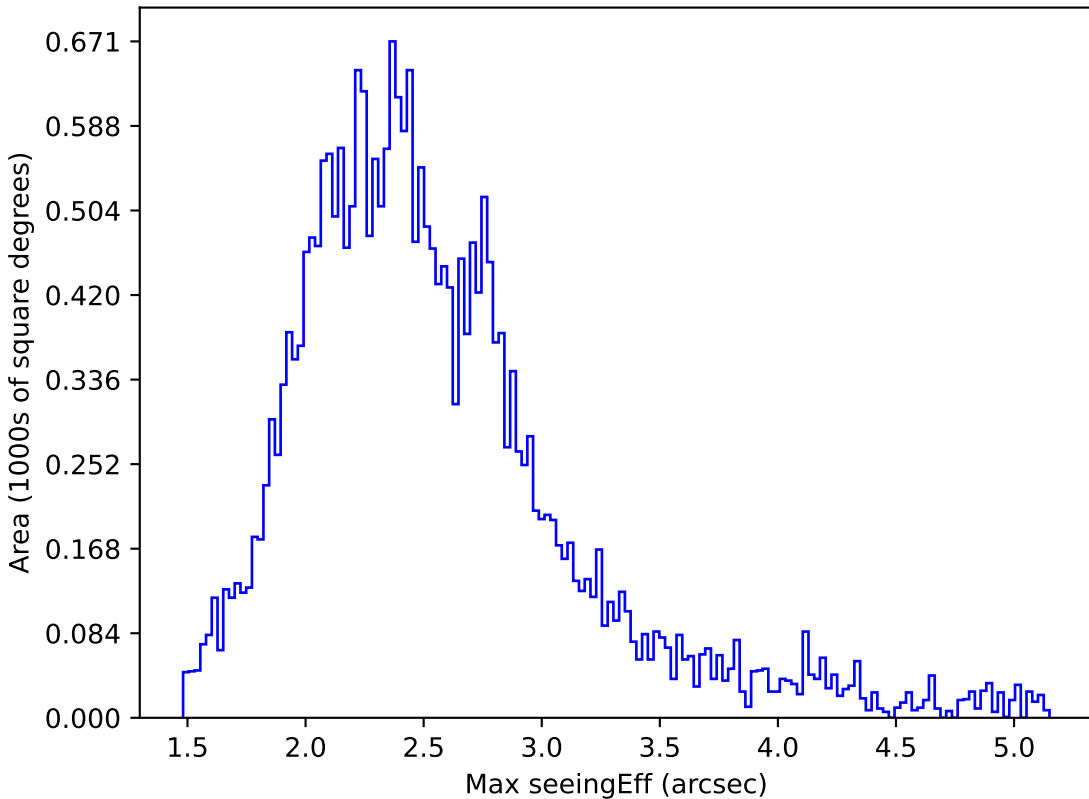
ddf_loaded_fl2_v3.4_10yrs All sky i band: Max seeingEff
