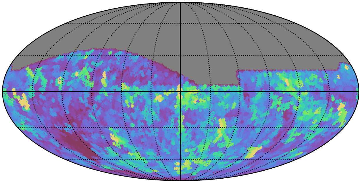
ddf_loaded_fl2_v3.4_10yrs All sky all bands: Max seeingEff
