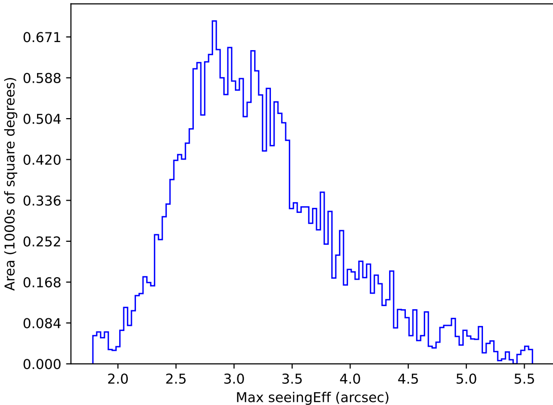
ddf_loaded_fl2_v3.4_10yrs All sky all bands: Max seeingEff
