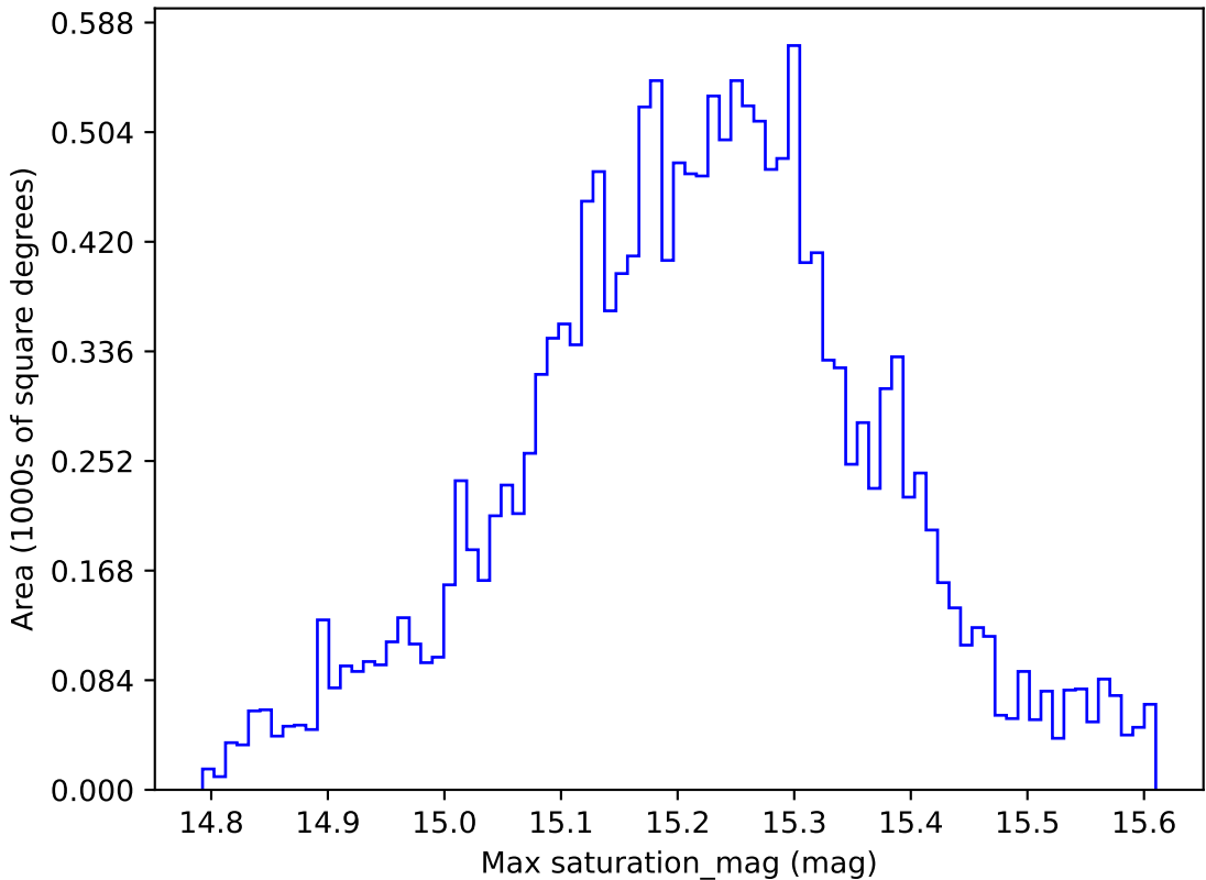
ddf_loaded_fl2_v3.4_10yrs WFD z band: Max saturation_mag
