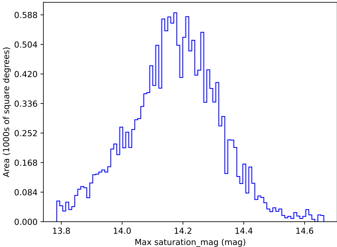
ddf_loaded_fl2_v3.4_10yrs WFD y band: Max saturation_mag
