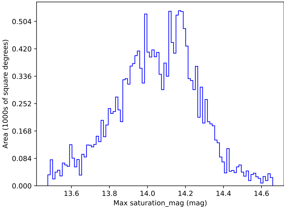
ddf_loaded_fl2_v3.4_10yrs WFD u band: Max saturation_mag
