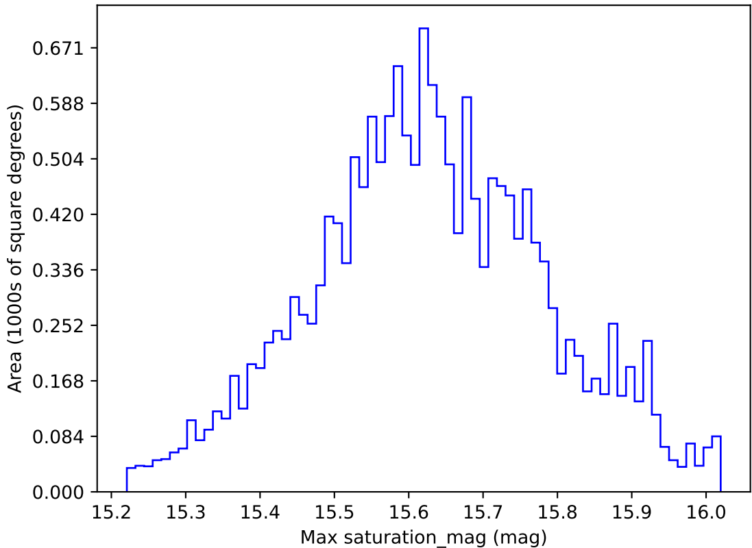
ddf_loaded_fl2_v3.4_10yrs WFD i band: Max saturation_mag
