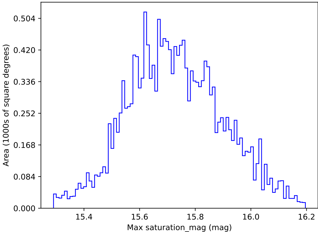
ddf_loaded_fl2_v3.4_10yrs WFD g band: Max saturation_mag
