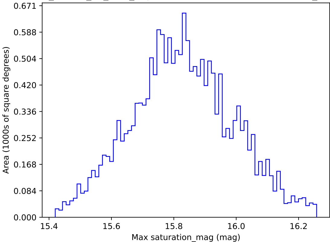
ddf_loaded_fl2_v3.4_10yrs WFD all bands: Max saturation_mag
