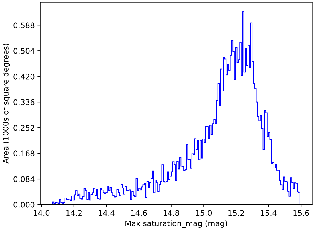
ddf_loaded_fl2_v3.4_10yrs All sky z band: Max saturation_mag
