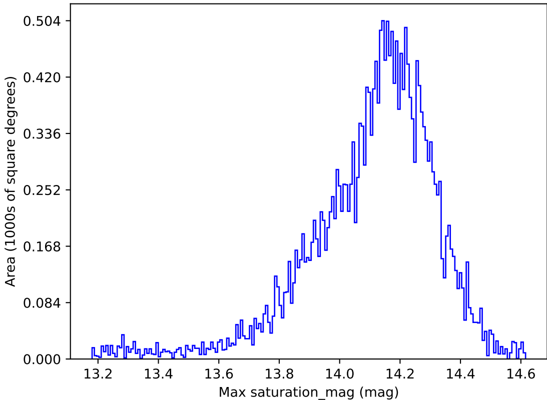
ddf_loaded_fl2_v3.4_10yrs All sky y band: Max saturation_mag
