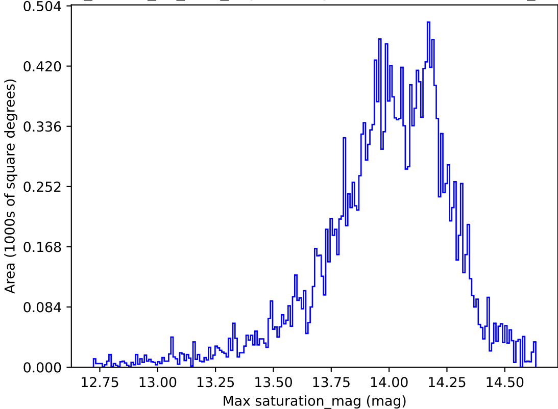
ddf_loaded_fl2_v3.4_10yrs All sky u band: Max saturation_mag
