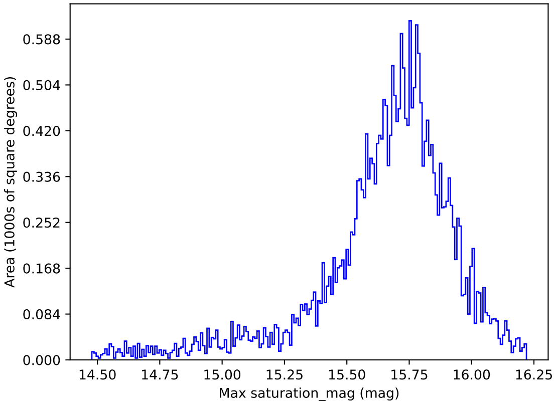
ddf_loaded_fl2_v3.4_10yrs All sky r band: Max saturation_mag
