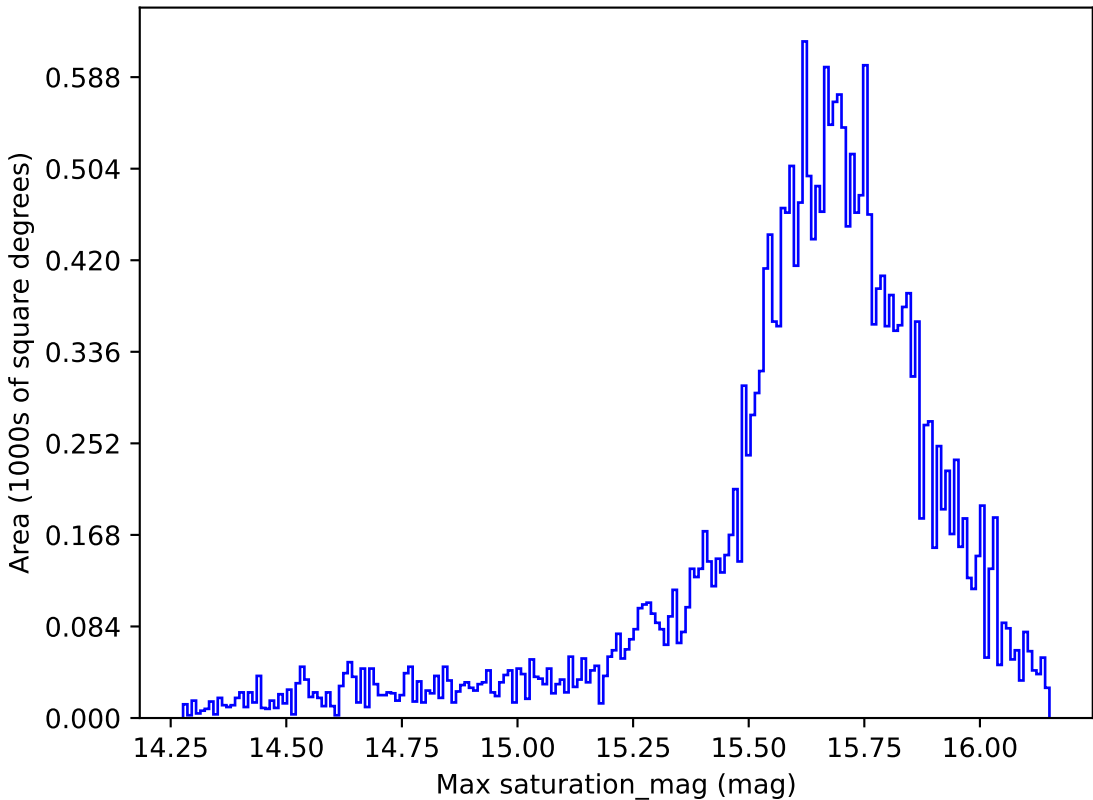
ddf_loaded_fl2_v3.4_10yrs All sky g band: Max saturation_mag
