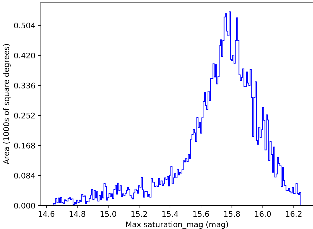
ddf_loaded_fl2_v3.4_10yrs All sky all bands: Max saturation_mag
