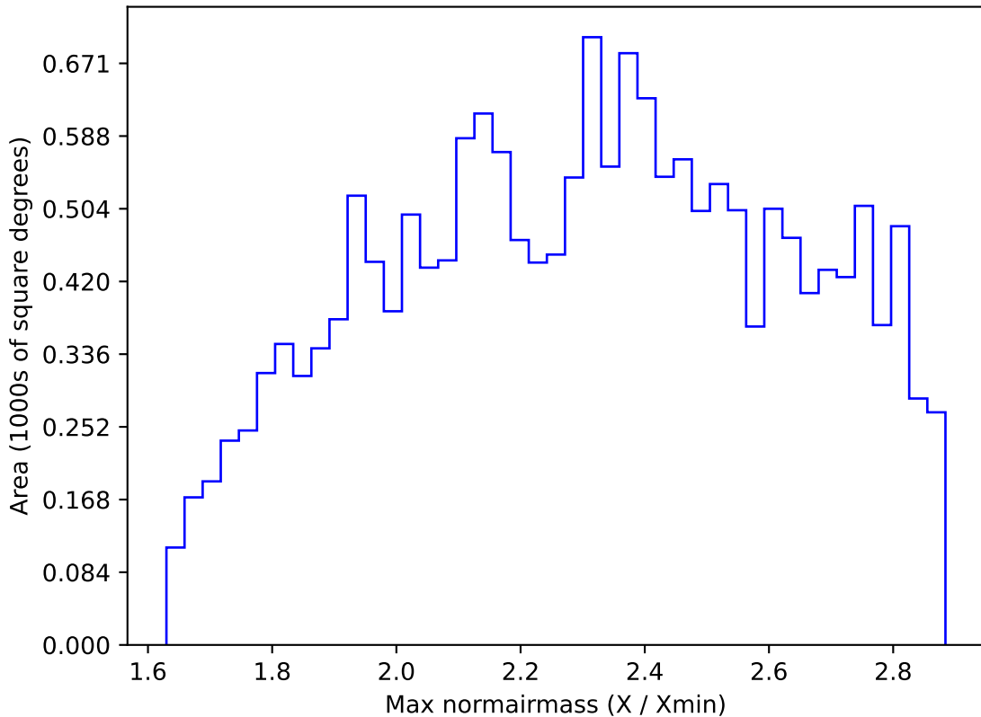
ddf_loaded_fl2_v3.4_10yrs WFD z band: Max normairmass
