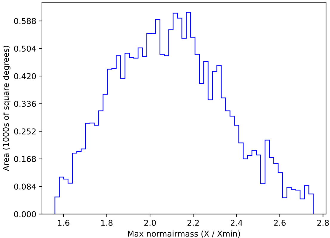
ddf_loaded_fl2_v3.4_10yrs WFD y band: Max normairmass
