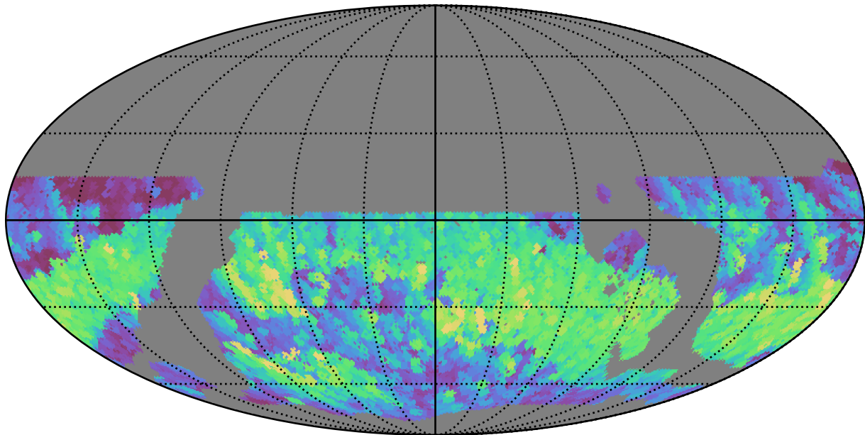
ddf_loaded_fl2_v3.4_10yrs WFD r band: Max normairmass
