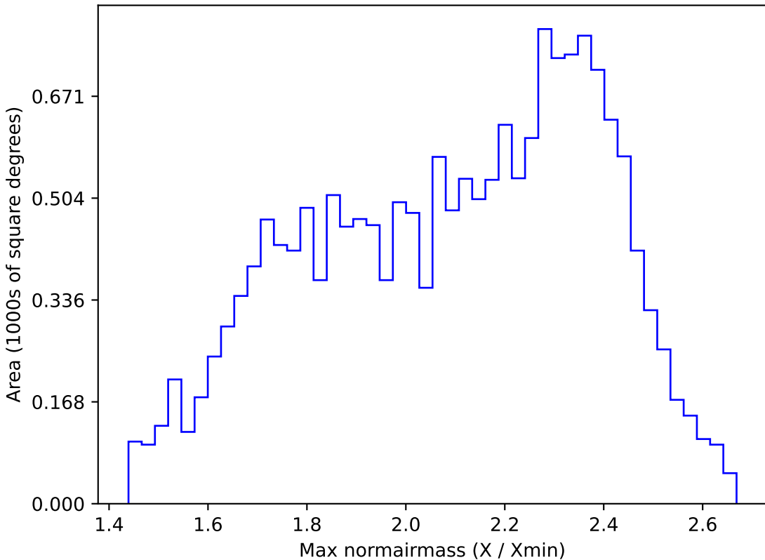
ddf_loaded_fl2_v3.4_10yrs WFD r band: Max normairmass
