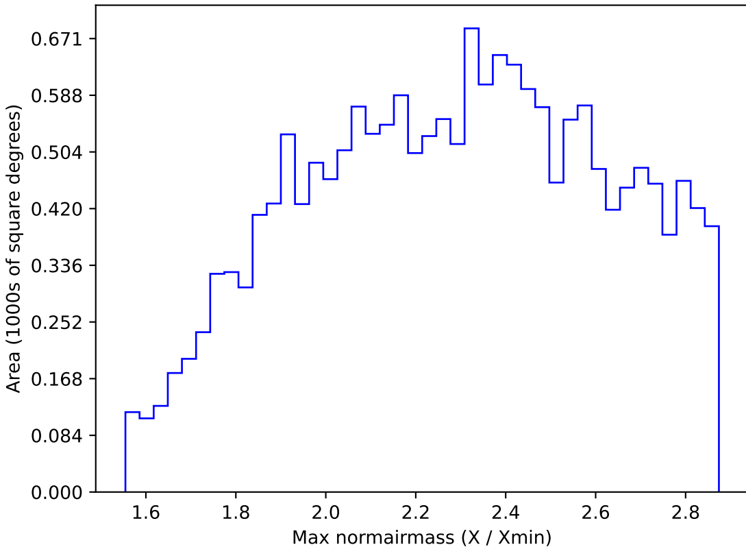
ddf_loaded_fl2_v3.4_10yrs WFD i band: Max normairmass
