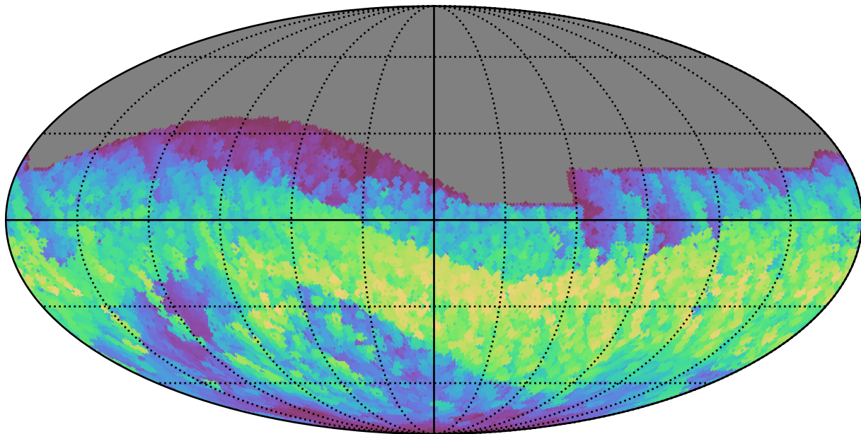
ddf_loaded_fl2_v3.4_10yrs All sky z band: Max normairmass
