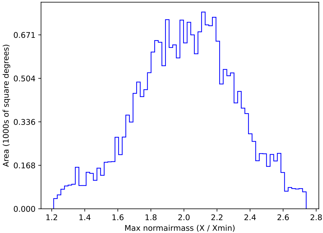
ddf_loaded_fl2_v3.4_10yrs All sky y band: Max normairmass
