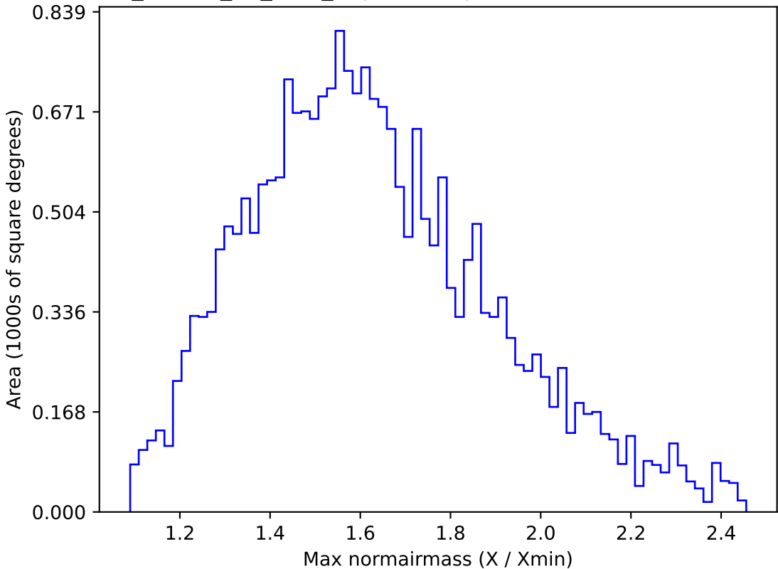
ddf_loaded_fl2_v3.4_10yrs All sky u band: Max normairmass
