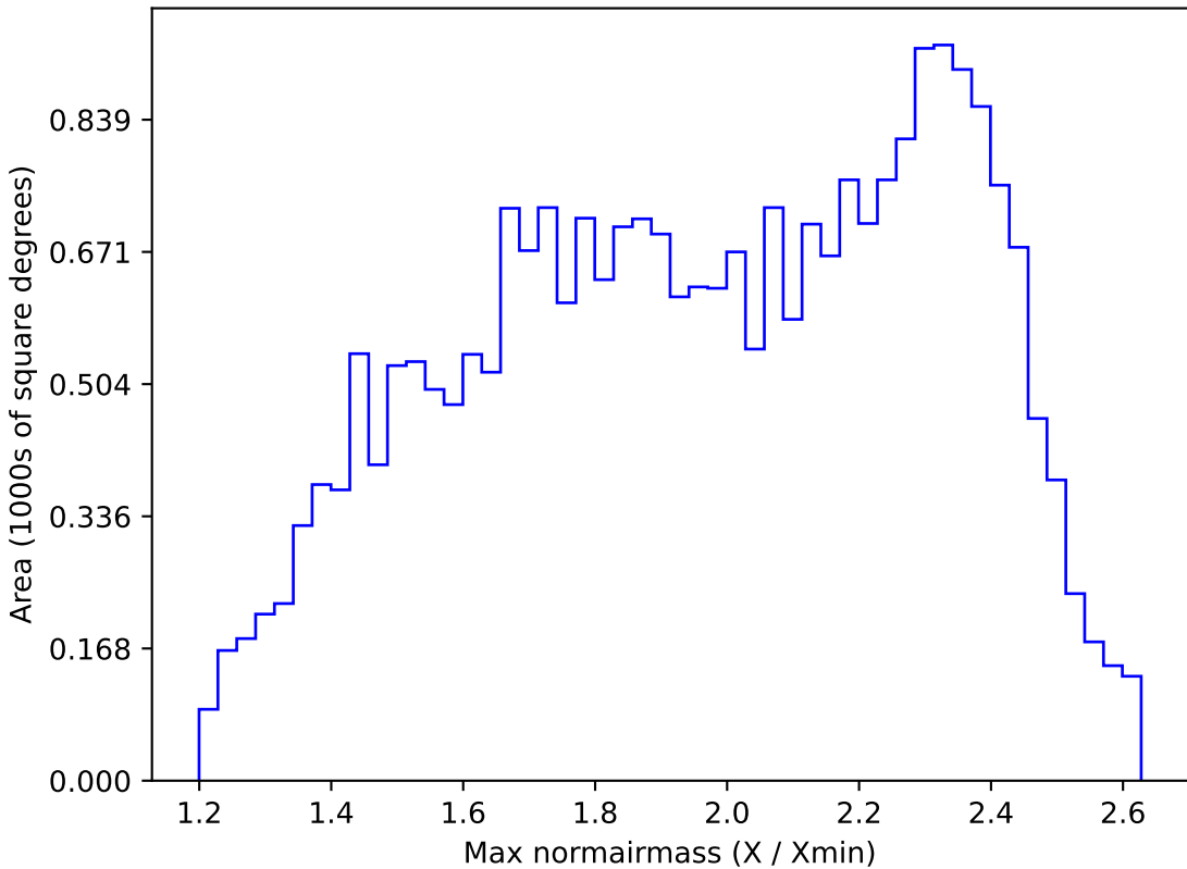
ddf_loaded_fl2_v3.4_10yrs All sky r band: Max normairmass
