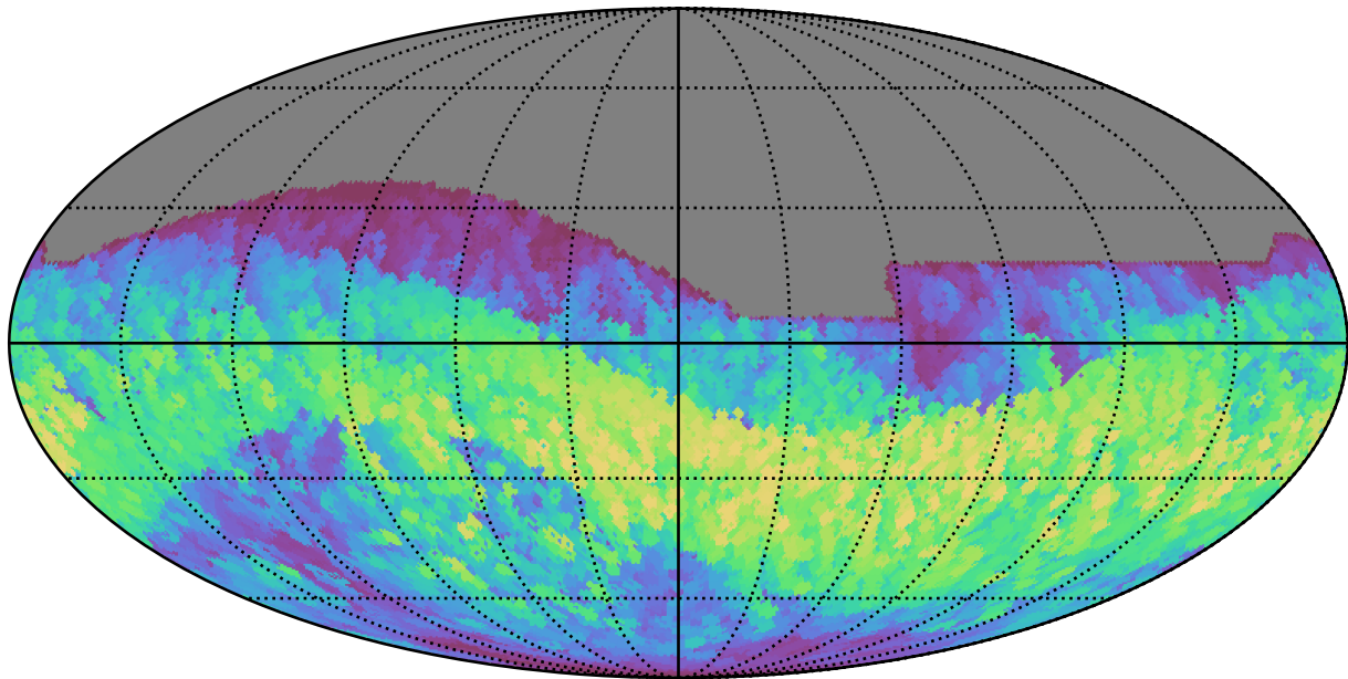
ddf_loaded_fl2_v3.4_10yrs All sky i band: Max normairmass
