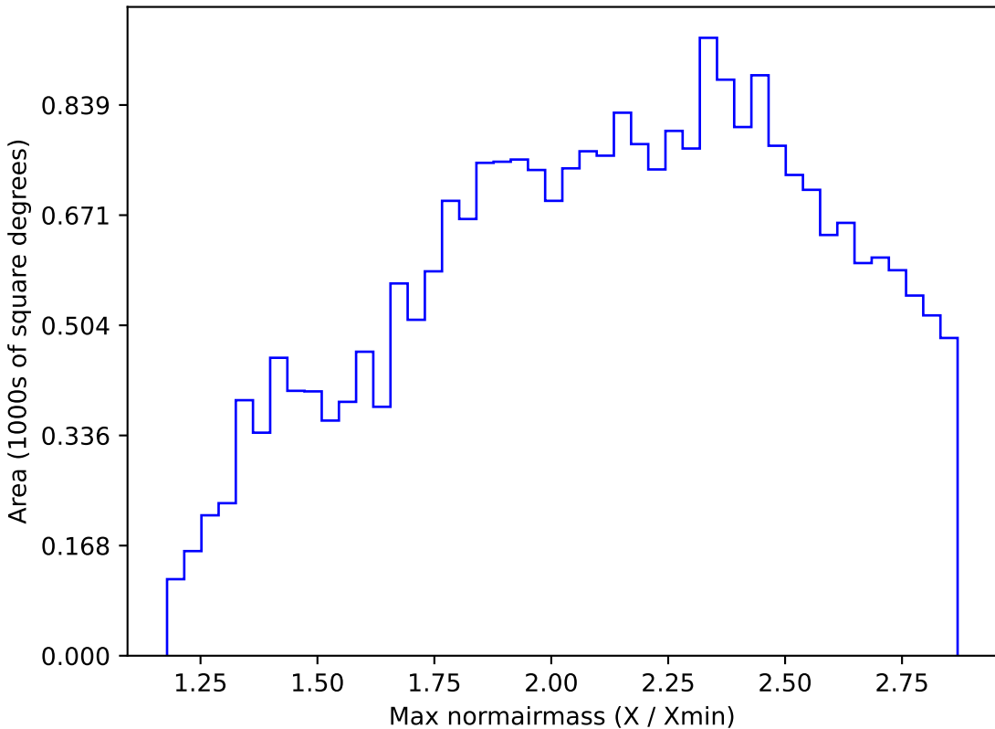
ddf_loaded_fl2_v3.4_10yrs All sky i band: Max normairmass
