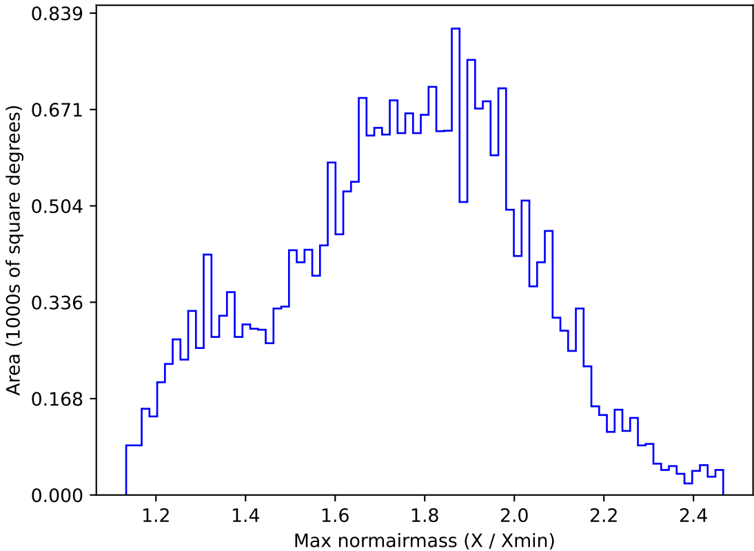
ddf_loaded_fl2_v3.4_10yrs All sky g band: Max normairmass
