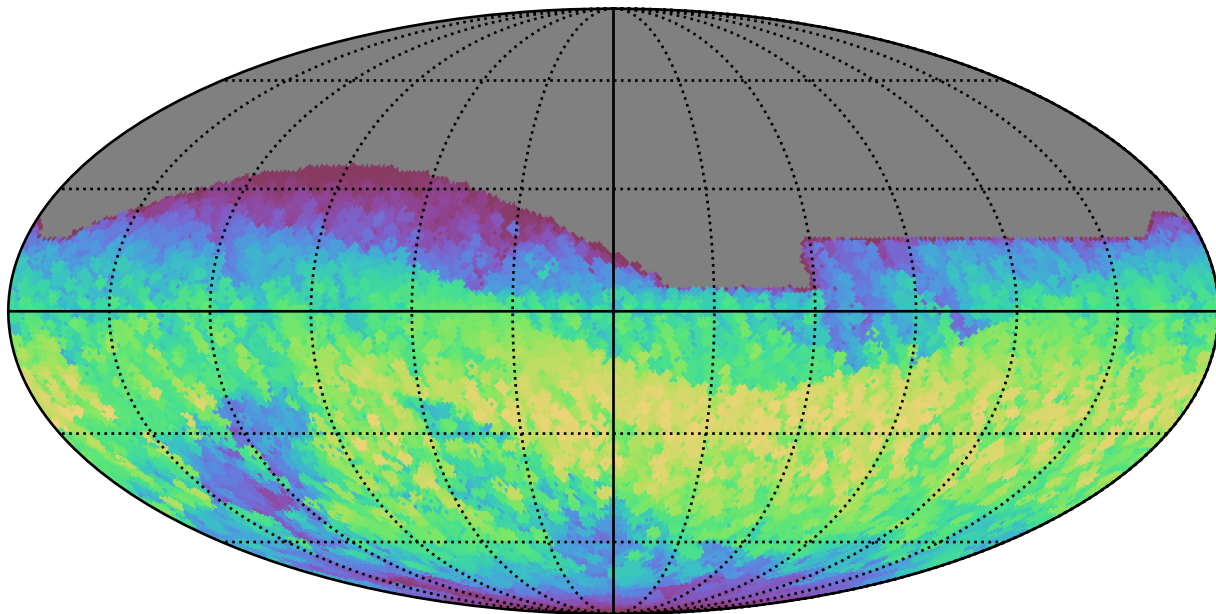
ddf_loaded_fl2_v3.4_10yrs All sky all bands: Max normairmass
