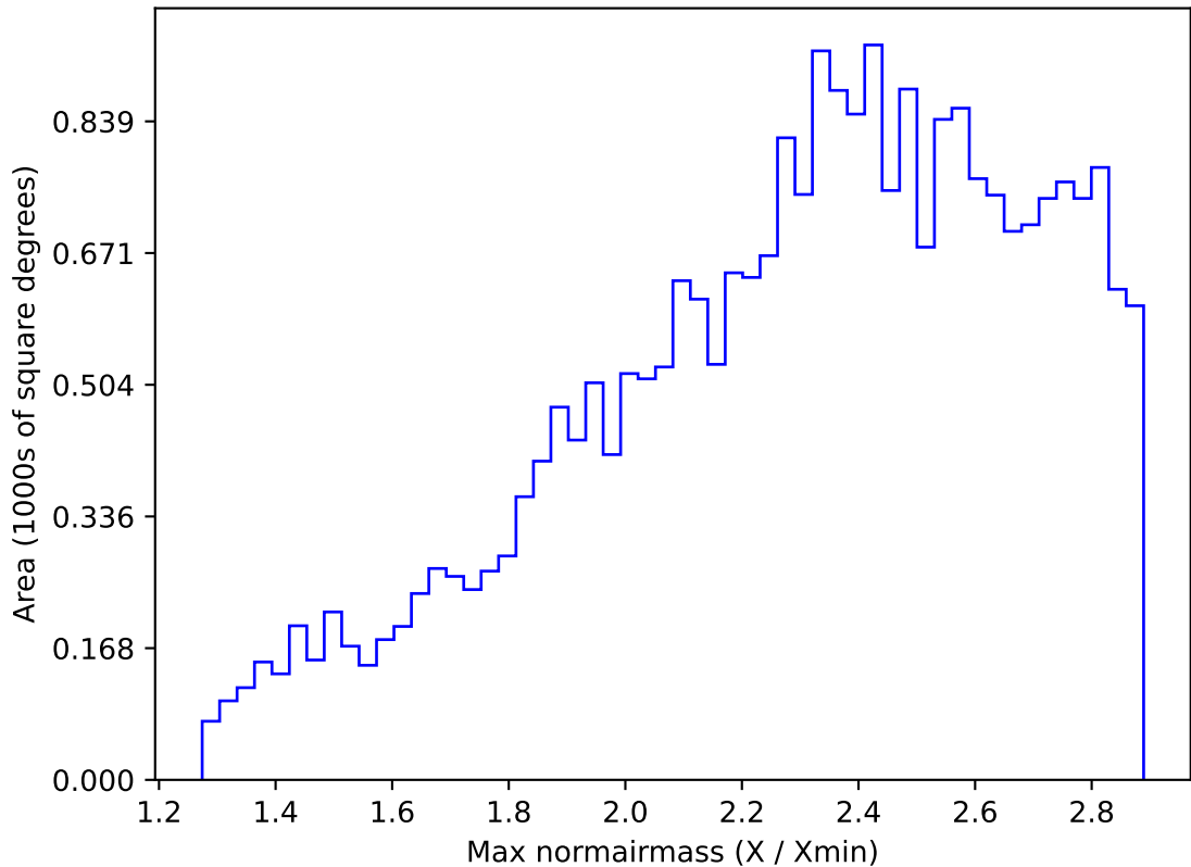
ddf_loaded_fl2_v3.4_10yrs All sky all bands: Max normairmass
