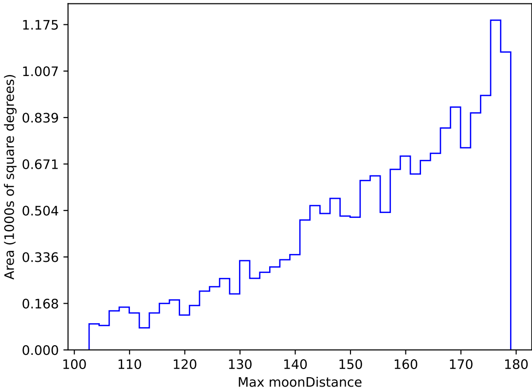
ddf_loaded_fl2_v3.4_10yrs WFD z band: Max moonDistance
