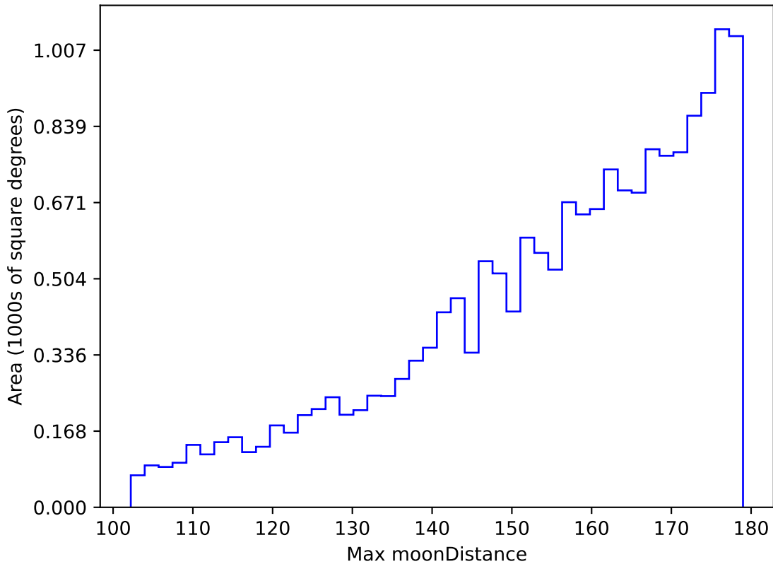
ddf_loaded_fl2_v3.4_10yrs WFD u band: Max moonDistance
