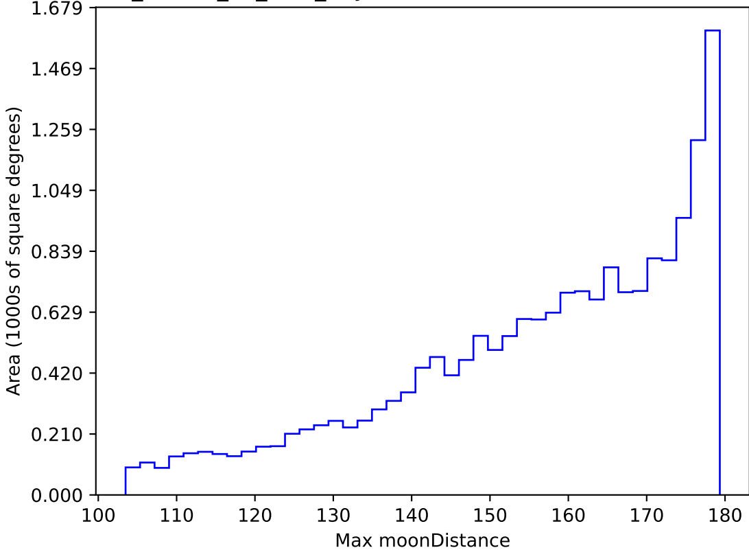
ddf_loaded_fl2_v3.4_10yrs WFD r band: Max moonDistance
