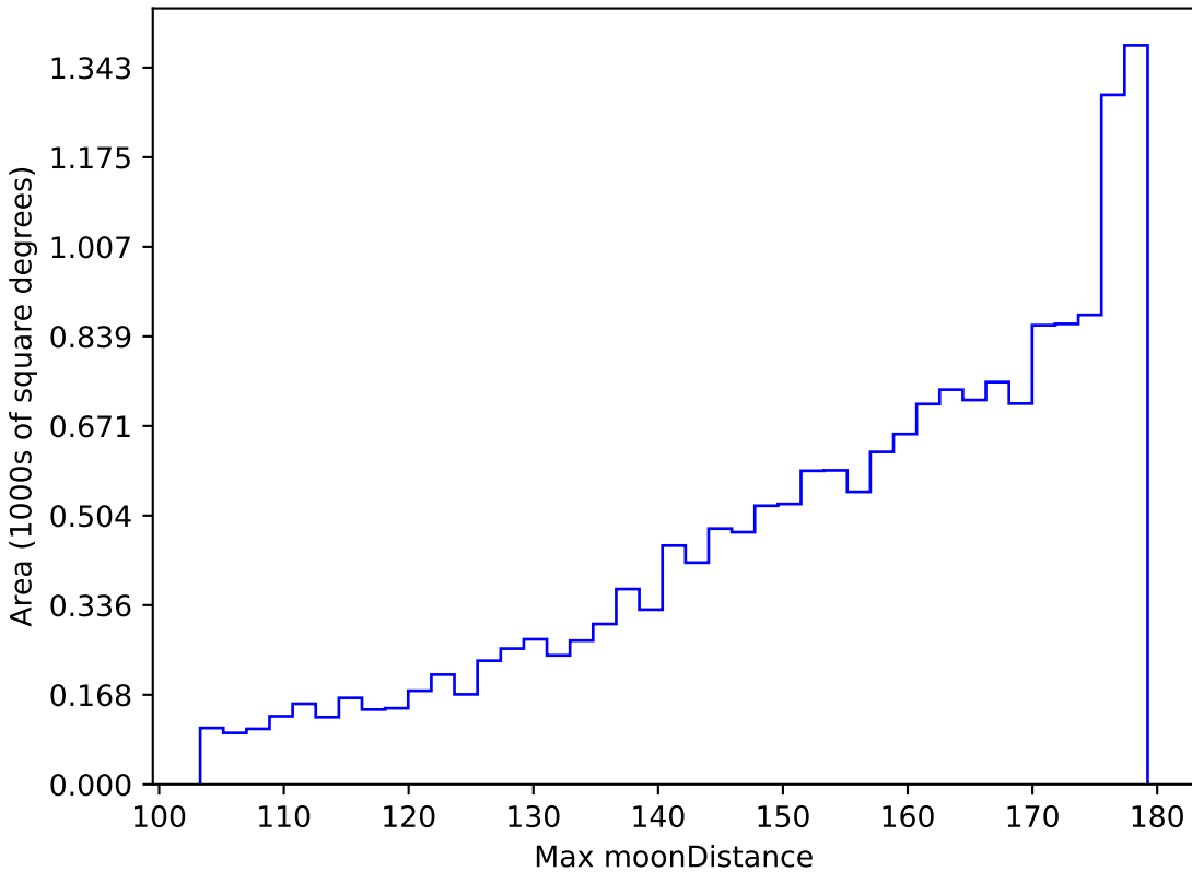
ddf_loaded_fl2_v3.4_10yrs WFD i band: Max moonDistance
