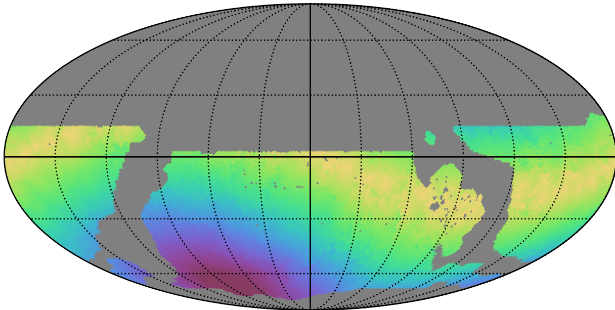
ddf_loaded_fl2_v3.4_10yrs WFD g band: Max moonDistance
