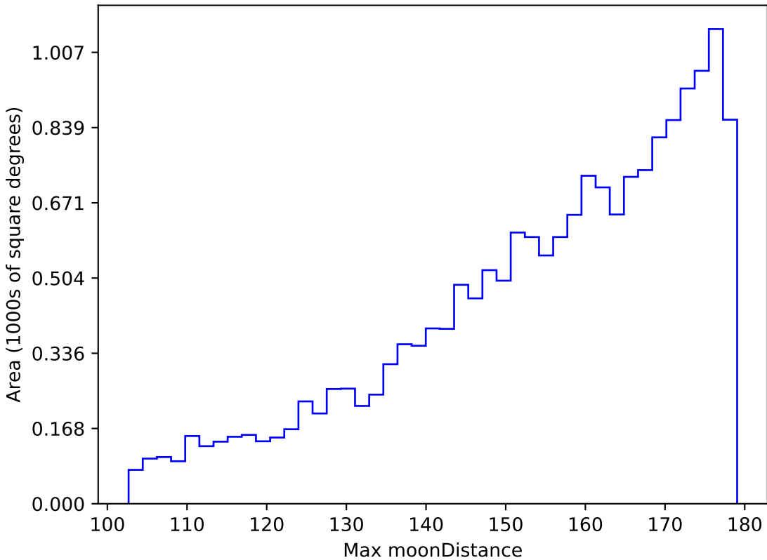
ddf_loaded_fl2_v3.4_10yrs WFD g band: Max moonDistance
