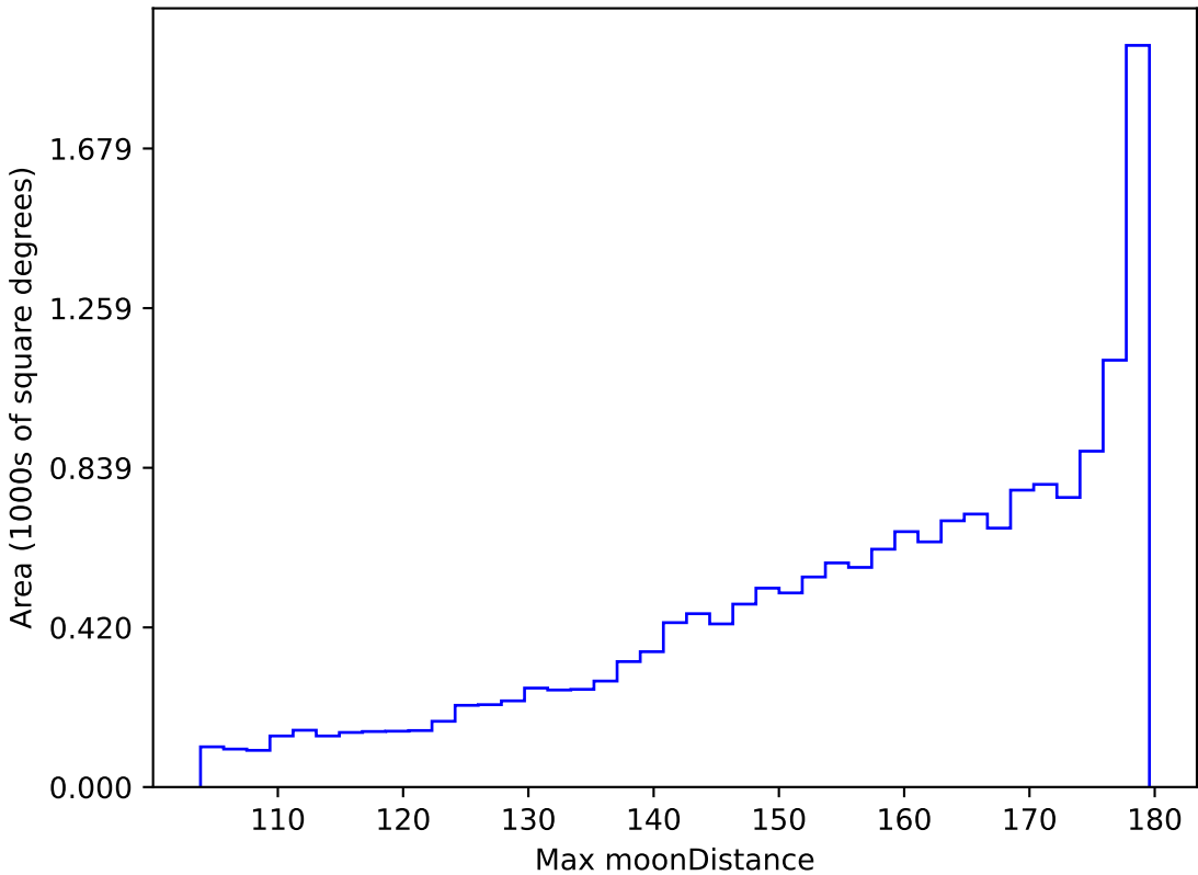
ddf_loaded_fl2_v3.4_10yrs WFD all bands: Max moonDistance
