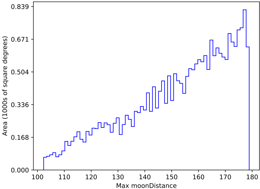
ddf_loaded_fl2_v3.4_10yrs All sky u band: Max moonDistance
