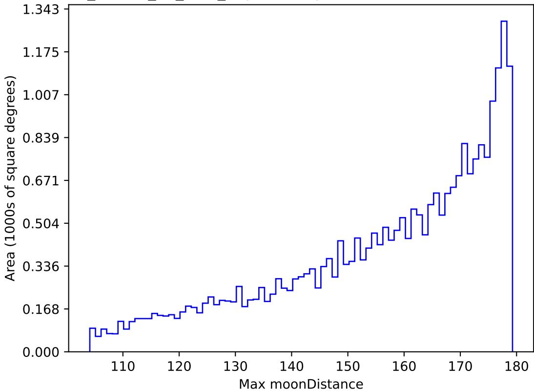
ddf_loaded_fl2_v3.4_10yrs All sky r band: Max moonDistance
